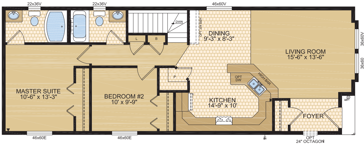
MAIN LEVEL
