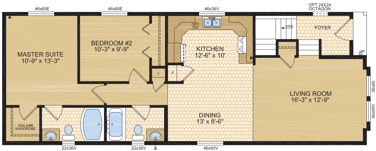
MAIN LEVEL
