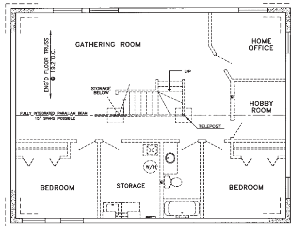
PROPOSED LOWER LEVEL
